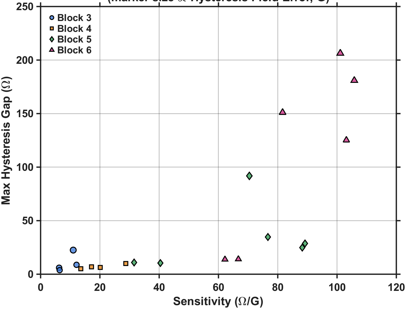
Sensitivity vs. Max Hysteresis Gap (marker size \propto Hysteresis Field Error, G)
